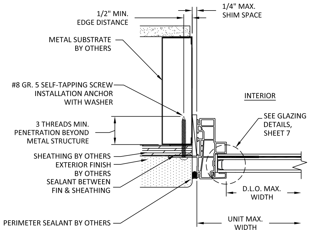
B 4 HORIZONTAL SECTION NAIL FIN INSTALLATION METAL SUBSTRATE
