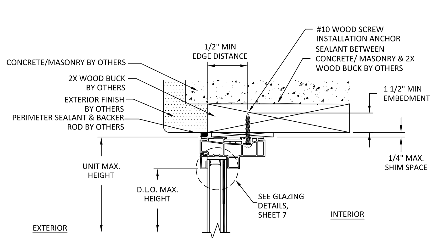
A 5 VERTICAL SECTION THROUGH FRAME INSTALLATION WOOD SUBSTRATE
