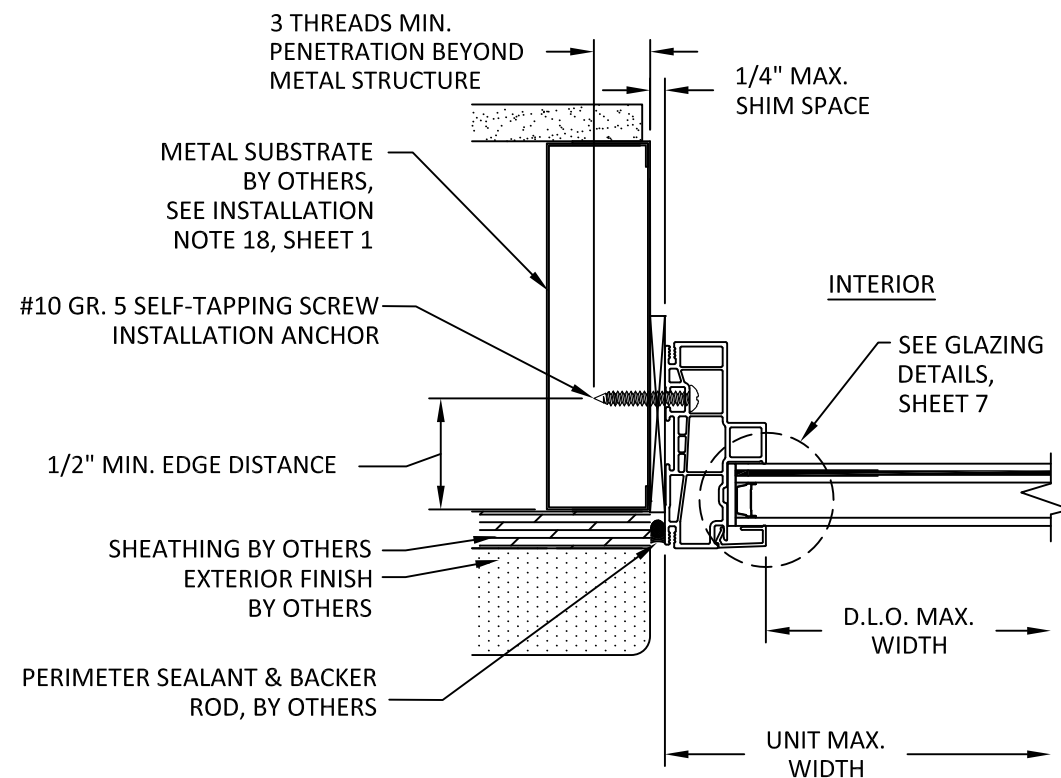
B 5 HORIZONTAL SECTION THROUGH FRAME INSTALLATION METAL SUBSTRATE
